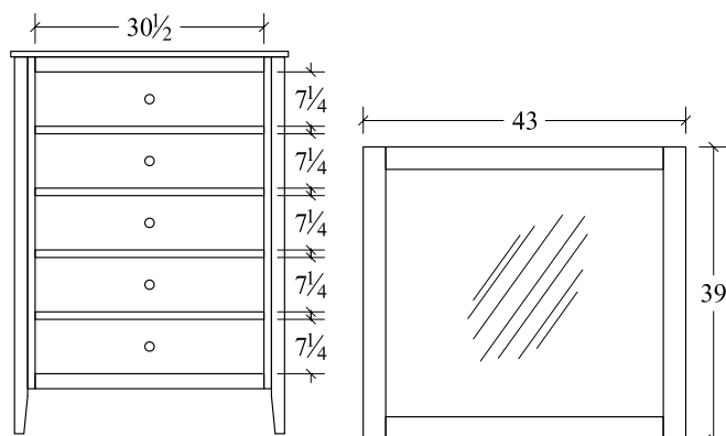
Chest (BNCD) 5 drawer 37w x 21 1/2d x 51h
