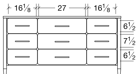
Dresser (ACDR9) 9 Drawer 68w x 18 3 / 4 d x 34 1 / 2 h
