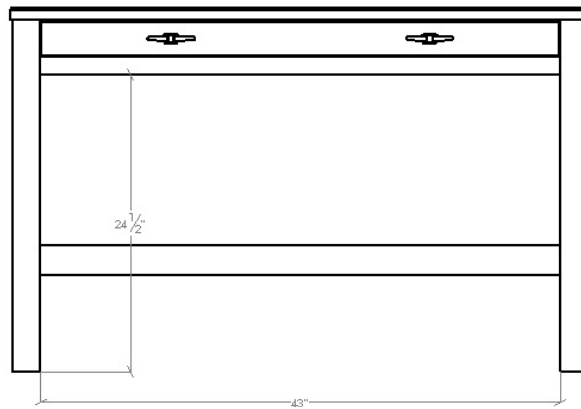
Platte River Writing Desk #PRDK48 48"W x 24"D x 30"H
