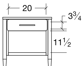
Nightstand (ACNS1) 1 Drawer 26w x 17d x 26 \frac{1}{4} h
