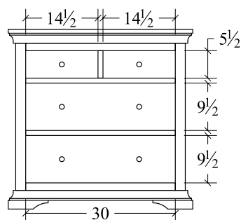
Chest (WTCD4) 4 drawer 37w x 22d x 36h
