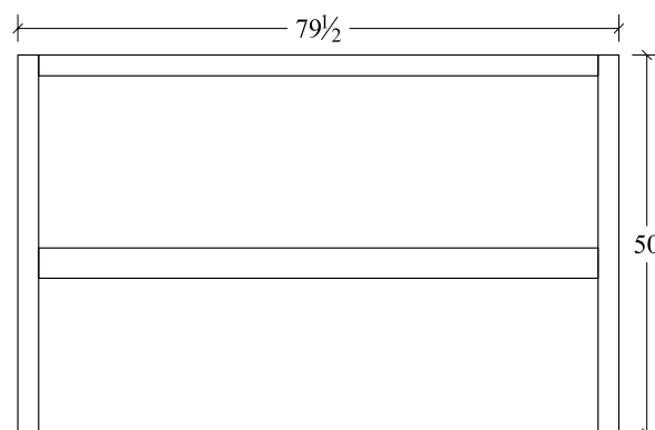
King Headboard (1-BNKB) 79 1/2w x 50h Queen Headboard (1-BNQB) 63 1/2w x 50h Full Headboard (1-BNFB) 57 1/2w x 50h Twin Headboard (1-BNTB) 42 1/2w x 50h Cal King Headboard (1-CBNKB) 75 1/2w x 50h
