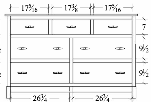
Dresser (PLDR) 7 drawer 60w x 21 1/2d x 38h
