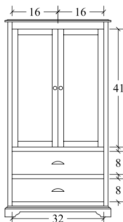
Armoire (EAAR) 2 drawer, 2 door 37w x 21 1/2d x 68 1/2h *2 shelves and 1 hanger rod
