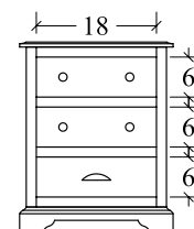
Night Stand (EANS3) 3 drawer 23w x 17d x 28 1/2h
