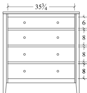
Chest (HECD4) 4 drawer 41w x 21 1/2d x 44h
