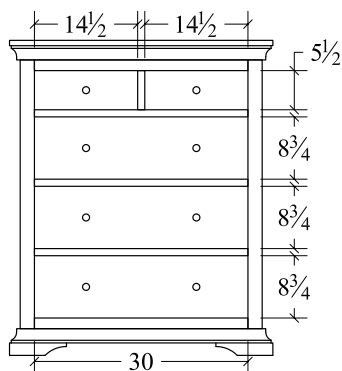
Chest (WTCD5) 5 drawer 37w x 22d x 44 3/4h
