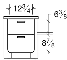
Nightstand (RSNS219) 2 drawer 19w x 16d x 25h
