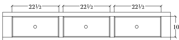
Storage Rail 3 drawer 14h
