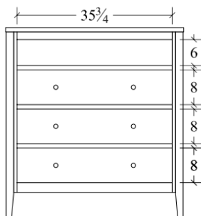
Media Chest (HEMC) 3 drawer, 1 opening 41w x 21 1/2d x 44h
