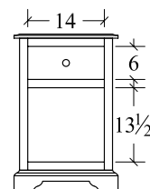
Night Stand (EANS119) 1 drawer 19w x 17d x 28 1/2h
