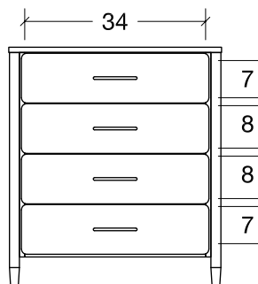
Chest (ACCD4) 4 Drawer 40w x 18 3 / 4 d x 45 1 / 2 h
