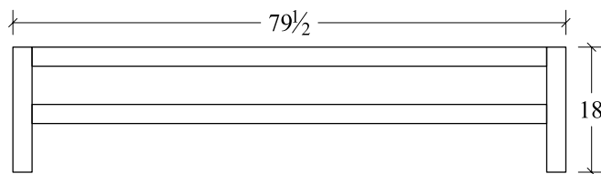
King Footboard (2-PRKB) 79 1/2w x 18h Queen Footboard (2-PRQB) 63 1/2w x 18h Full Footboard (2-PRFB) 57 1/2w x 18h Twin Footboard (2-PRTB) 42 1/2w x 18h Cal King Footboard 2-CPRKB 75 1/2w x 18h
