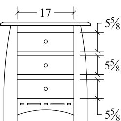
Nightstand (HYNS) 3 drawer 27w x 18d x 30h
