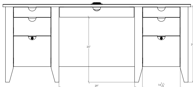
Simplicity 72 inch Drawer Desk #SPDK72DT 72"w x 30"d x 30"h
