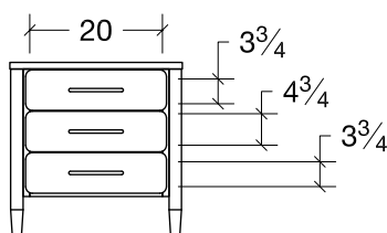
Nightstand (ACNS3) 3 Drawer 26w x 17d x 26 \frac{1}{4} h
