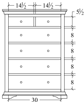
Chest (WTCD) 6 drawer 37w x 22d x 51h
